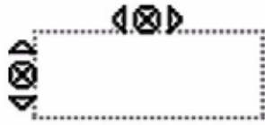
Figure 181 Cell Icons
