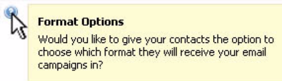
Figure 5 Tooltips
