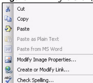
Figure 177 Right-Click (Image)
