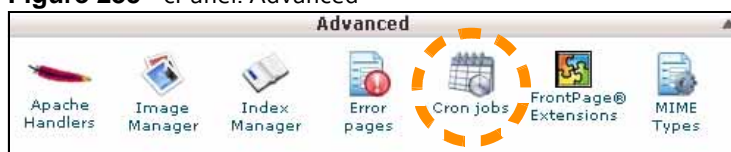
Figure 235 cPanel: Advanced
