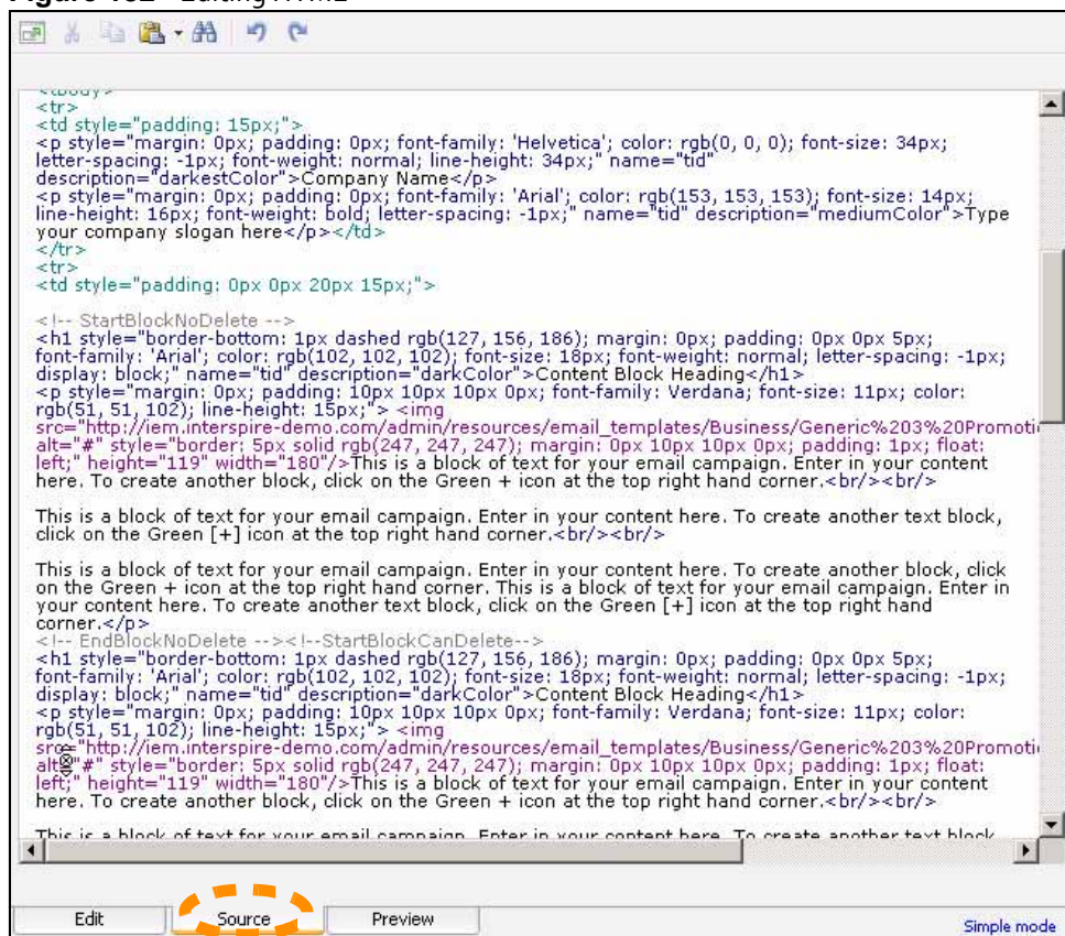
Figure 182 Editing HTML
