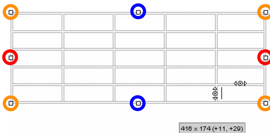
Figure 180 Table Icons
