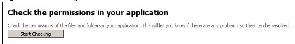
Figure 246 Checking Permissions
