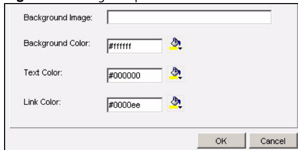
Figure 173 Page Properties
