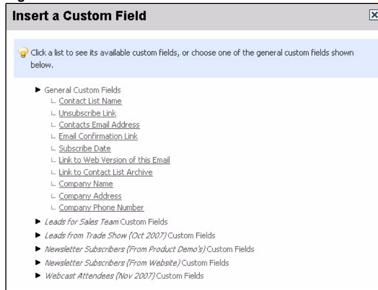
Figure 174 Custom Fields
