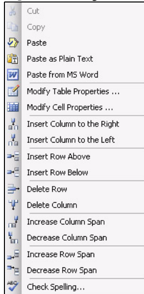
Figure 179 Right-Click (Table)
