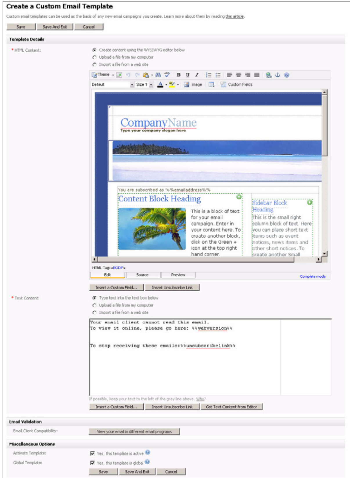
Figure 199 The Template Editor
