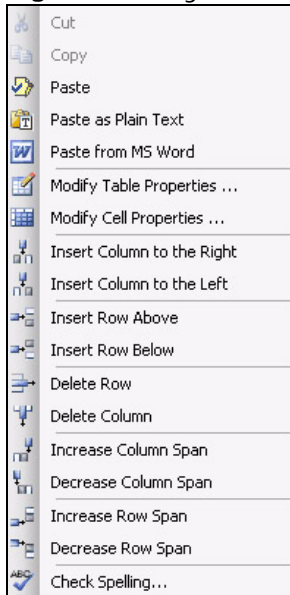
Figure 176 Right-Click (Text)
