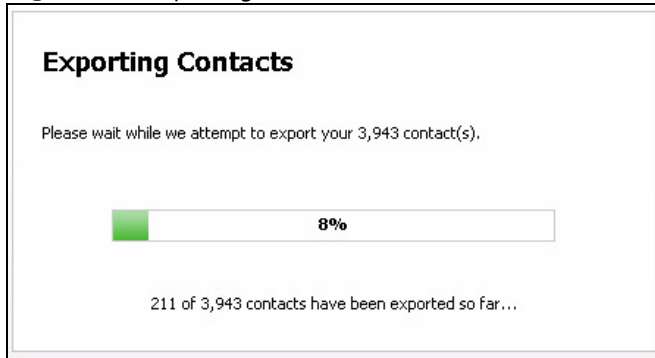
Figure 53 Exporting Contacts
