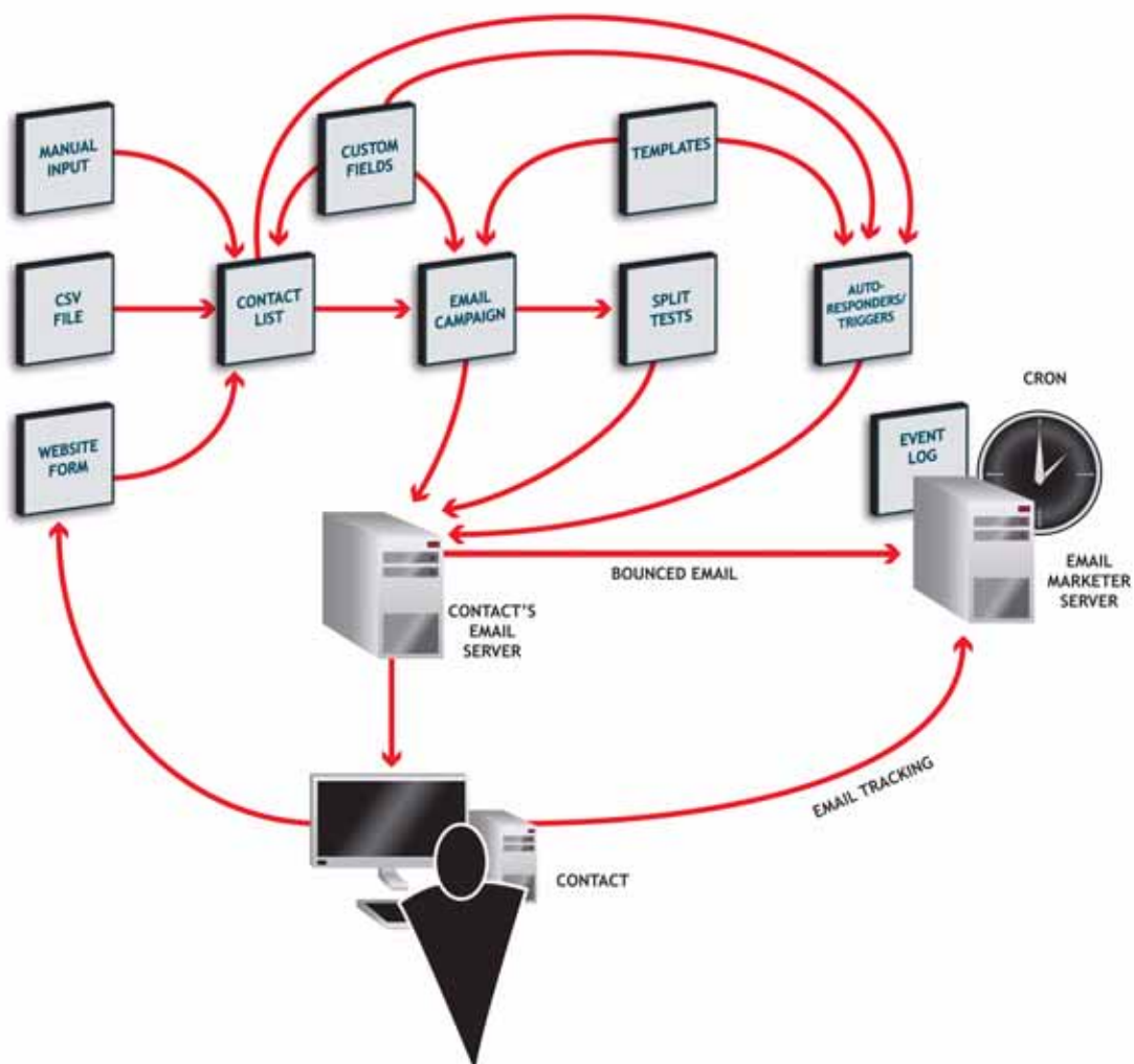
Figure 1 Interspire Email Marketer Overview
